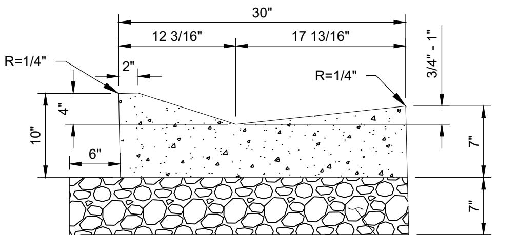
TYPE 2 (MOUNTABLE)
